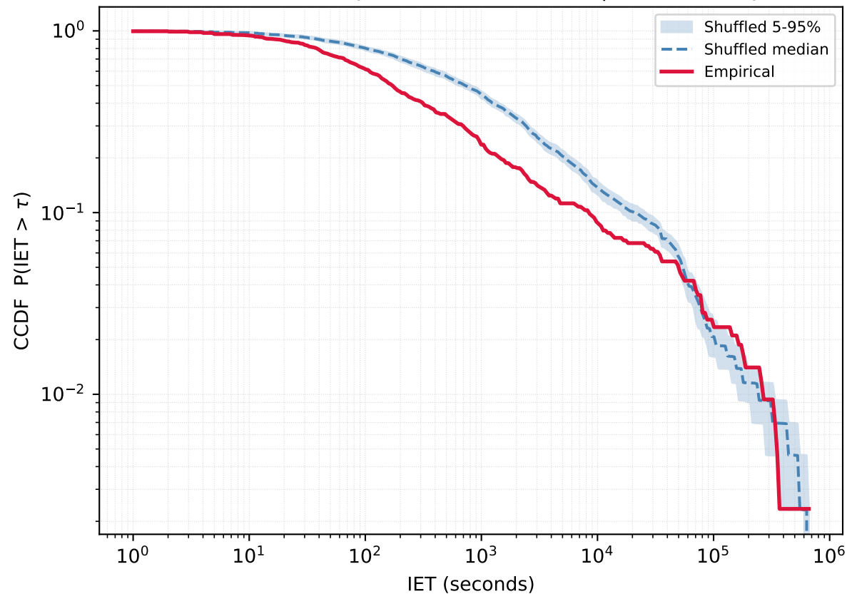
User 1762777403 - Empirical vs Reshuffled | KS=0.248 p=0.000
